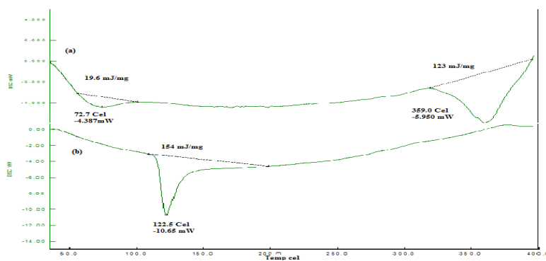
Figure 2. DSC of omeprazole-PVP crystals (a) pure omeprazole (b)
